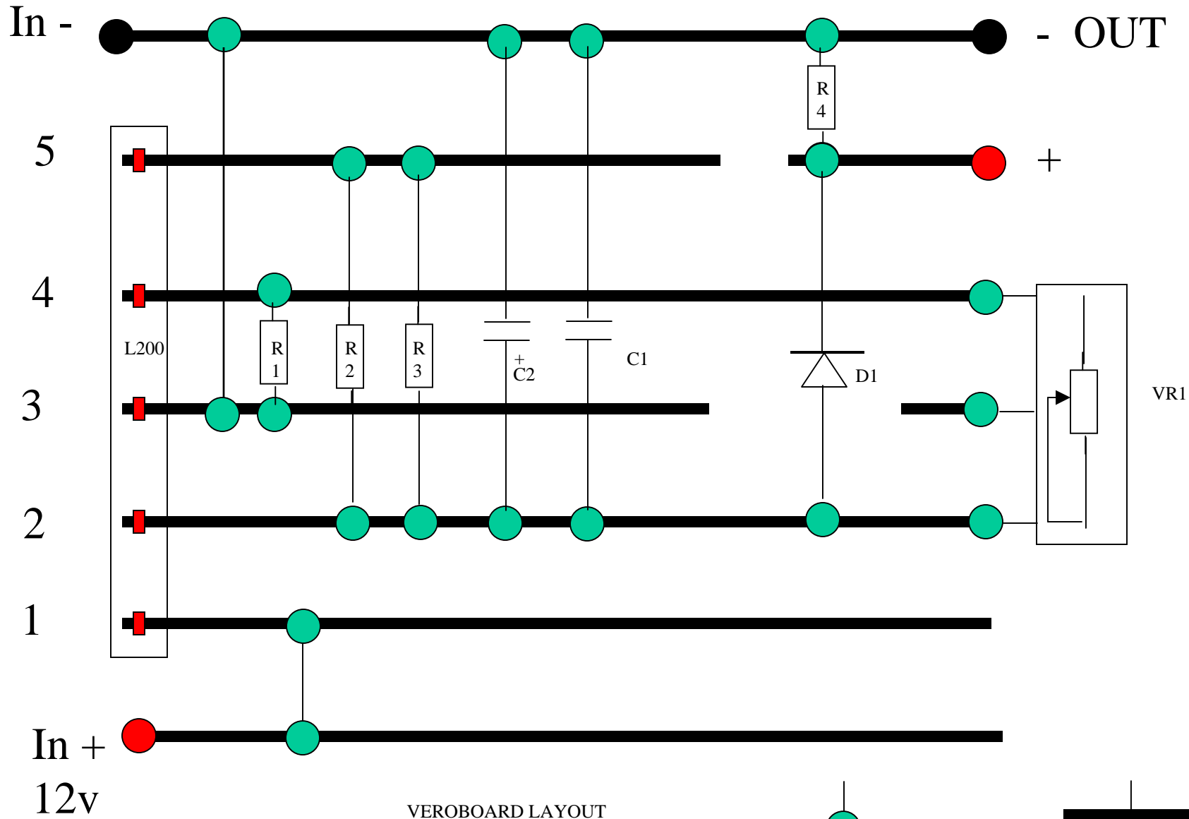
VEROBOARD LAYOUT
